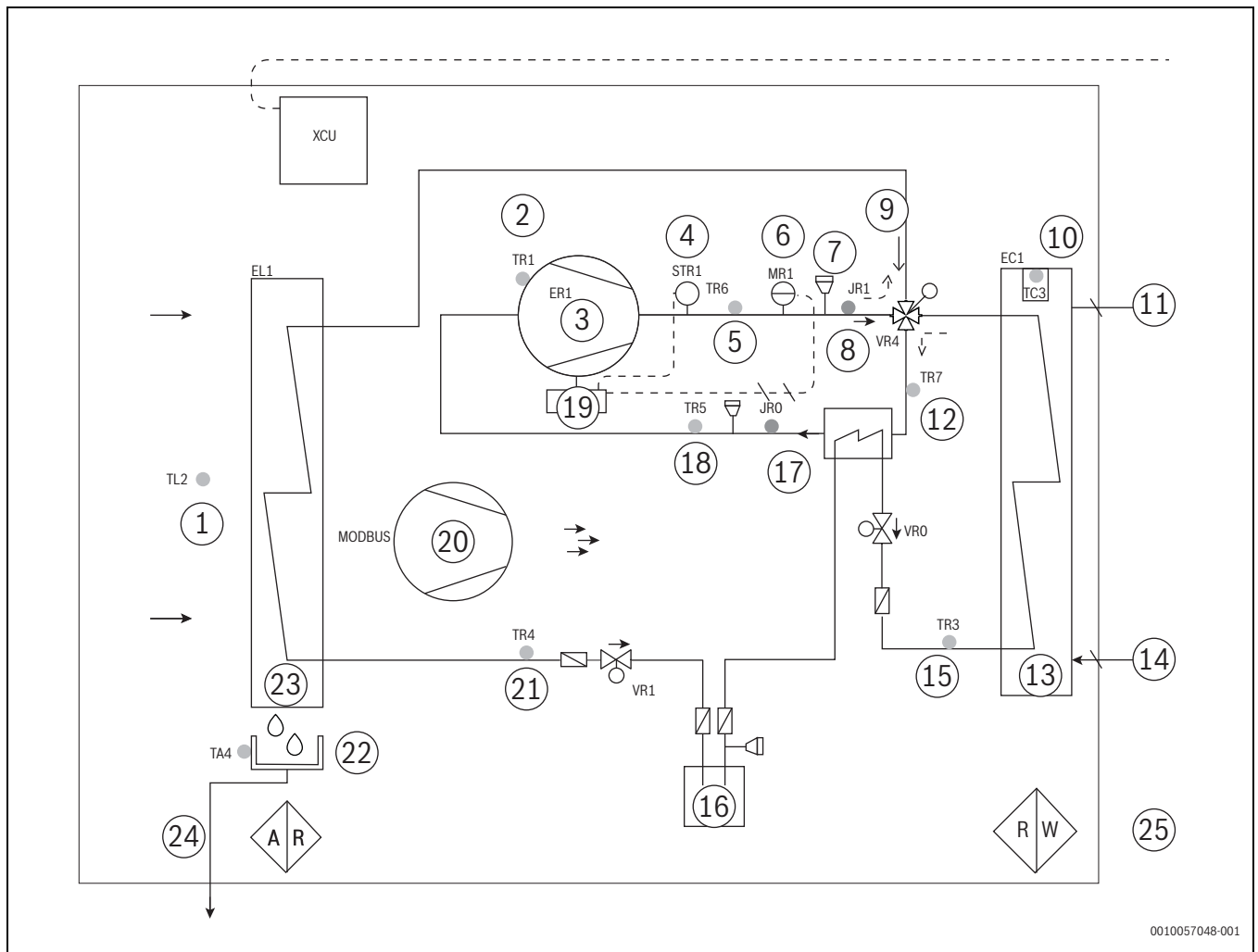
Fig. 13 Refrigerant circuit
